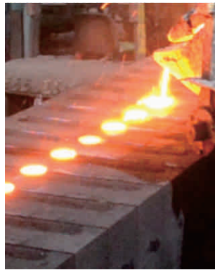
铁水浇铸 Hot Metal Pouring Into The Tooling
